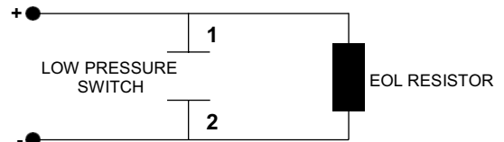
LOW PRESSURE SWITCH WIRING
