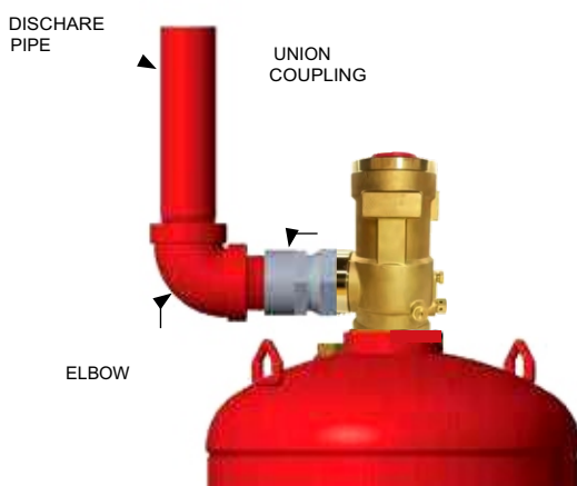
8 L THROUGH 180 L CONTAINERS: Part No. 300008
