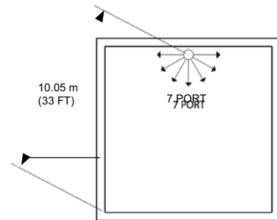
1 NOZZLE DISCHARGE RADIUS
