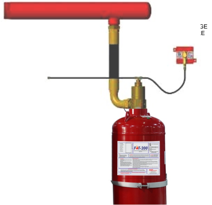
DISCHARGE PRESSURE SWITCH INSTALLATION (MULTIPLE CONTAINER SYSTEM)
